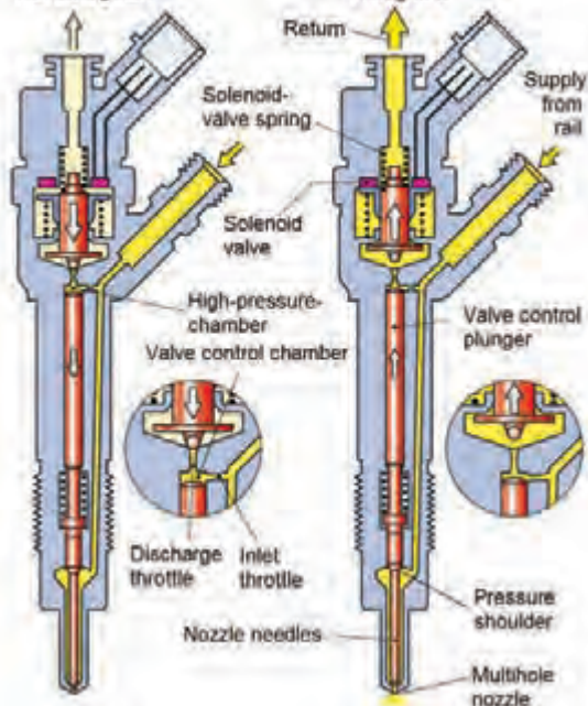
Solenoid valve not energised
